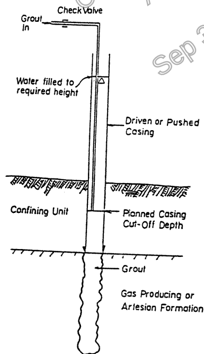
Stand Pipe To Contain Excess Formation Pressure
