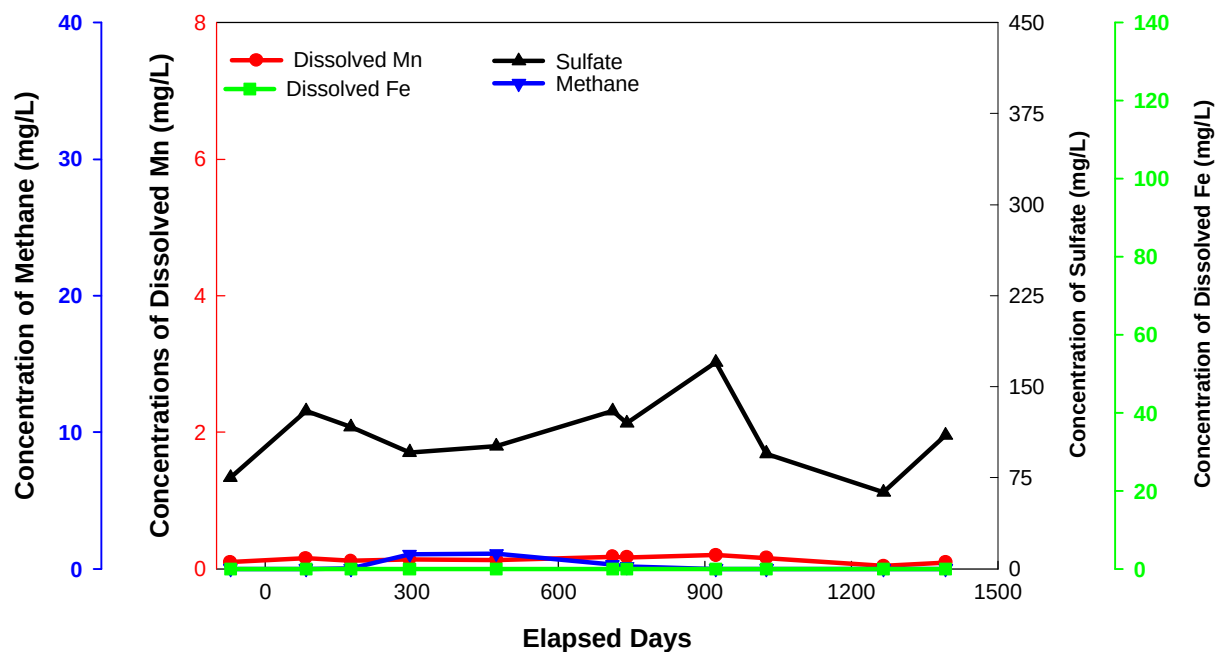
Figure E-16. Bioattenuation Parameters at GM-32 - Downgradient Well in RZ-3 West
