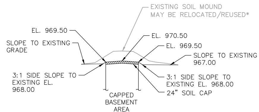
2 4 NORTH-SOUTH CROSS SECTION
