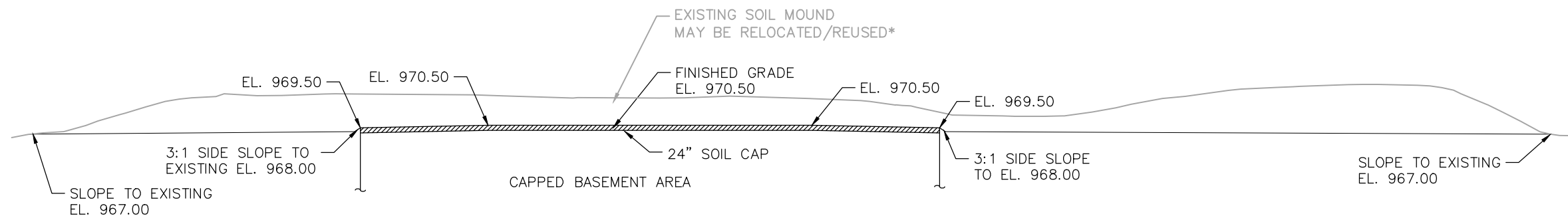
1 4 EAST-WEST CROSS SECTION
