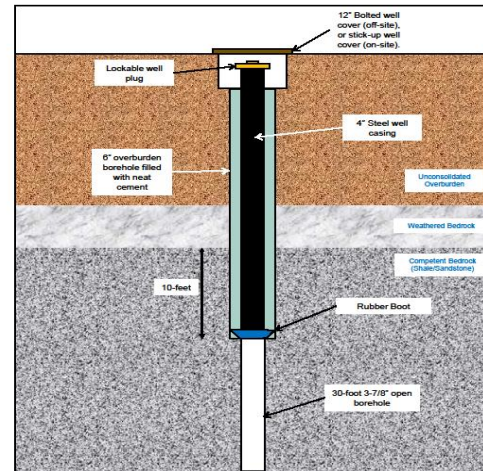
Figure 2 Bedrock Monitoring Well Schematic RACER Trust, Plants 2, 3 & 6, Lansing, Michigan
