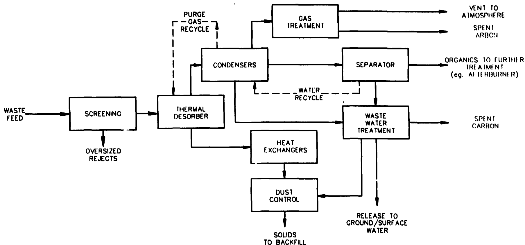
figure 5.15 THERMAL DESORPTION PROCESS GENERAL FLOW DIAGRAM TEXTILE ROAD SITE Washtenaw County, Michigan
