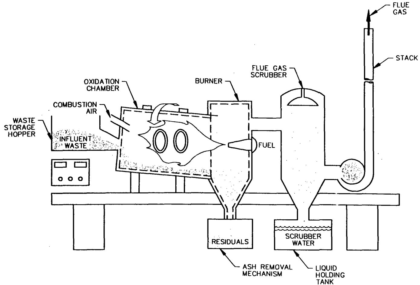
figure 5.14 OFF-SITE INCINERATION SCHEMATIC OF ROTARY KILN TEXTILE ROAD SITE. Washtenaw County, Michigan
