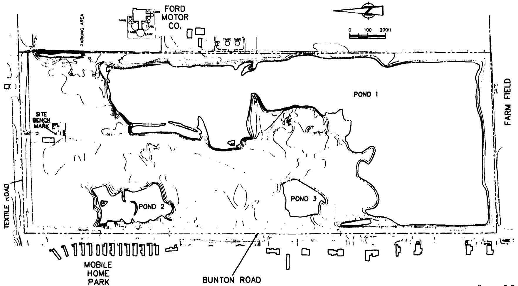
figure 2.2 SITE PLAN TEXTILE ROAD SITE Washtenaw County, Michigan
