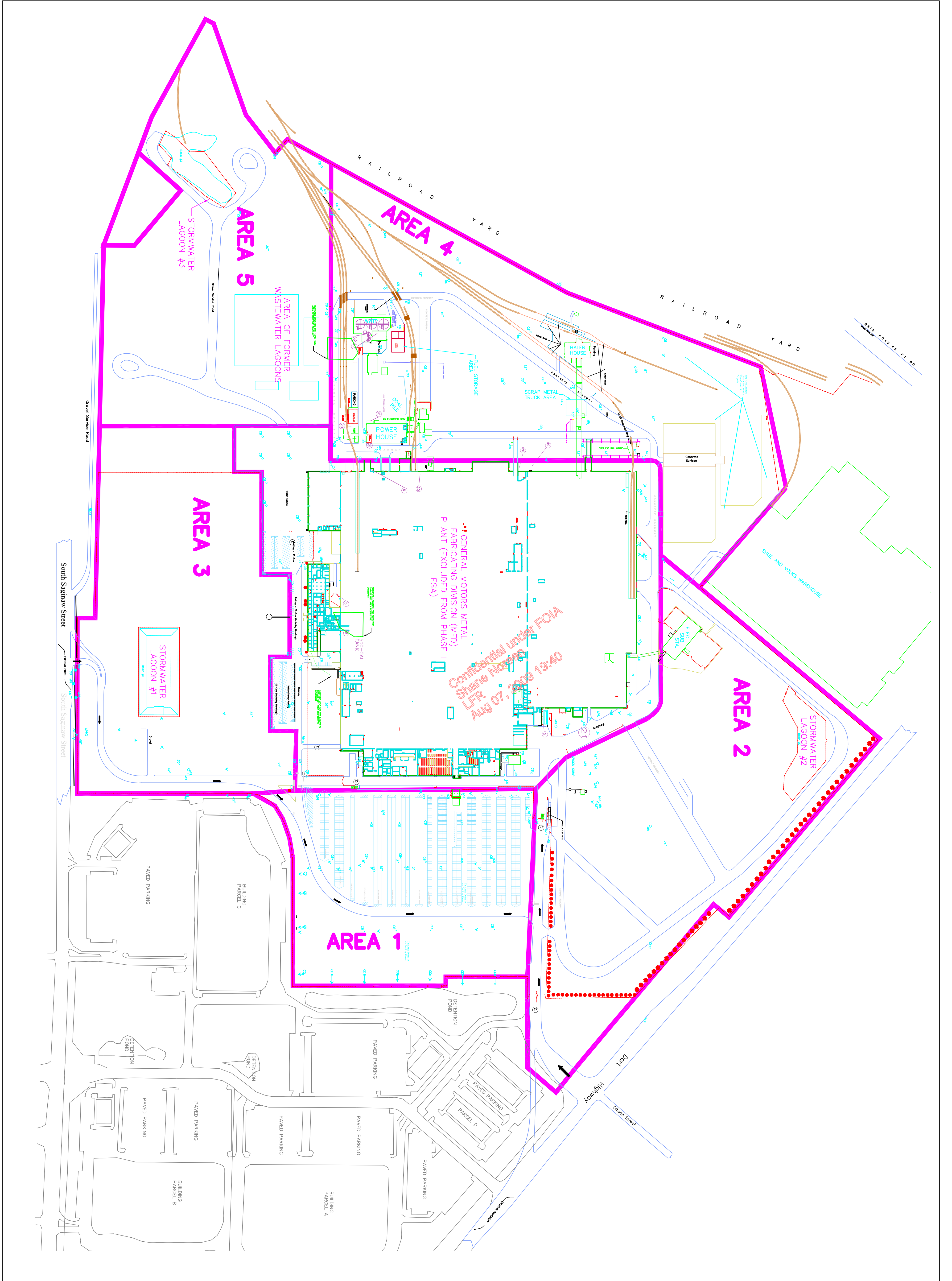
SITE LAYOUT GENERAL MOTORS MFD - GRAND BLANC (SITE #29) GRAND BLANC, MICHIGAN
